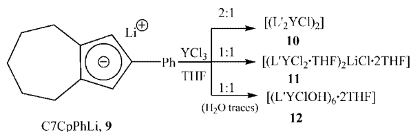
Scheme 2. Synthesis of the 2-phenyl-substituted complexes.
