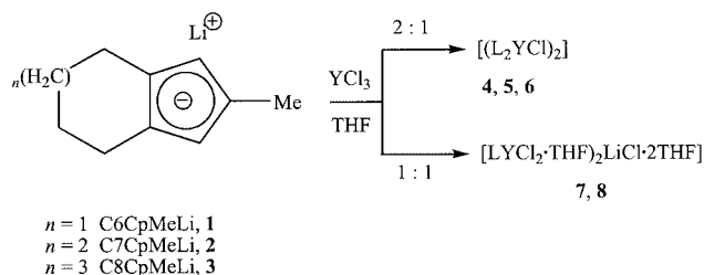
Scheme 1. Synthesis of the 2-methyl-substituted complexes.
