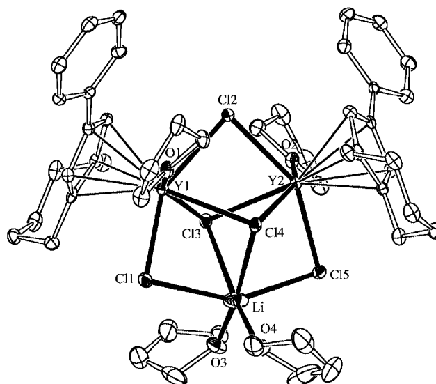
Figure 1. ORTEP [10] view of complex 11 displaying the thermal ellipsoids at 30% probability. The hydrogen atoms have been omitted for sake of clarity.
