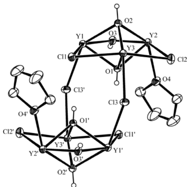
Figure 3. Diagram of the metal, halogen, and hydroxy framework of complex 12 , including the coordinated THF molecules.
