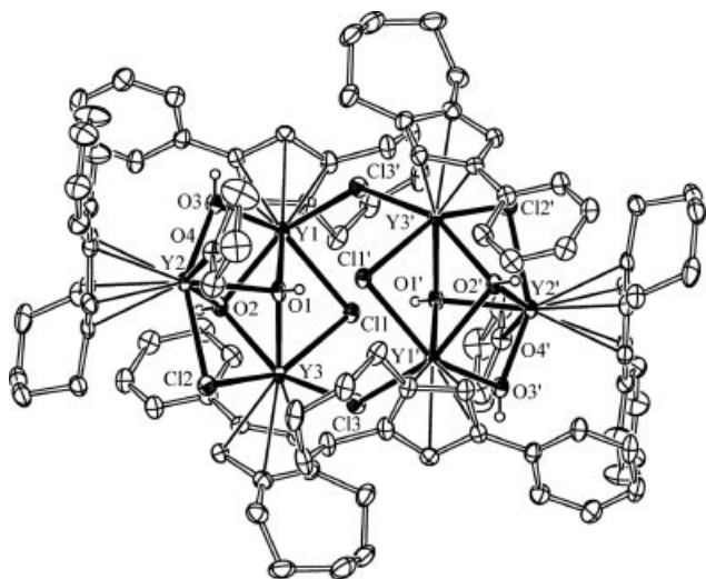
Figure 2. ORTEP view of complex 12 displaying the thermal ellipsoids at 30% probability. The hydrogen atoms have been omitted for sake of clarity.
